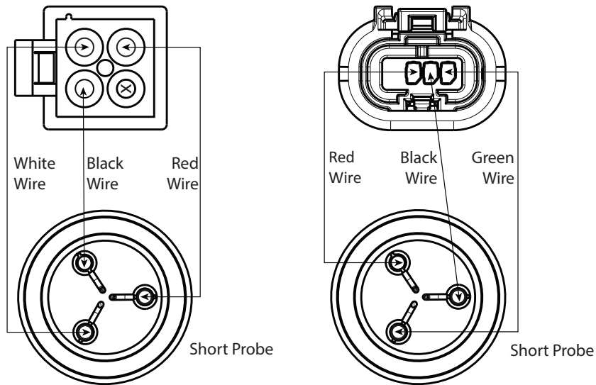
Ohm Water Level Probe and Wiring Harness
