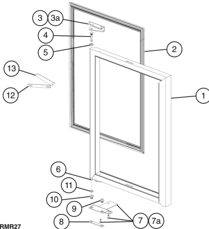
Title: F. Door-Left Glass Door Hinged Models: Undercounter, Worktop, Prep Table
