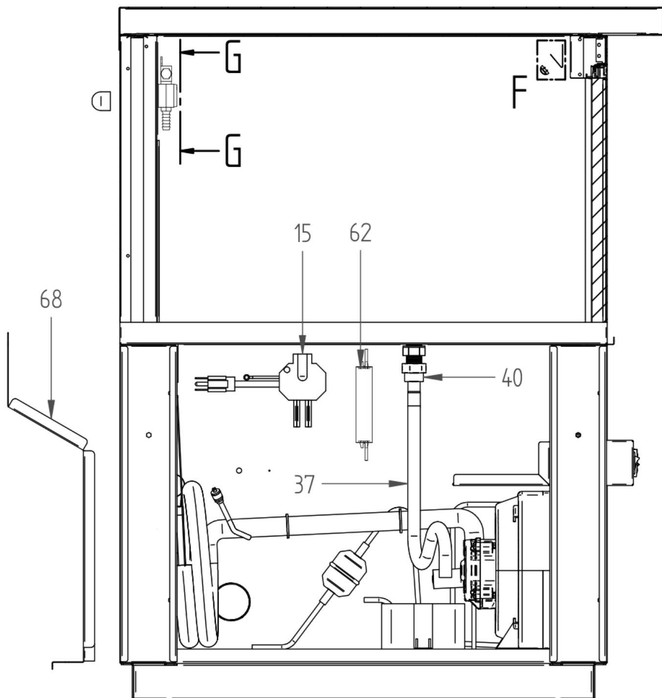
DETAIL F
