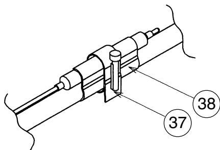
EXPANSION VALVE BULB HOLDER DETAIL
