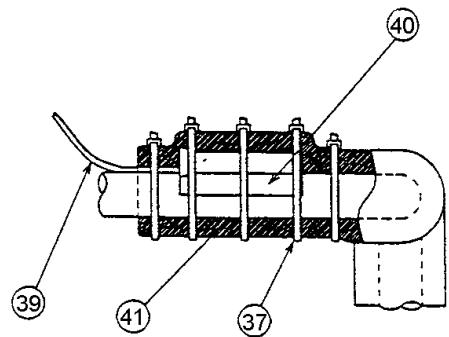
DETAILED THERMISTOR ATTACHM
