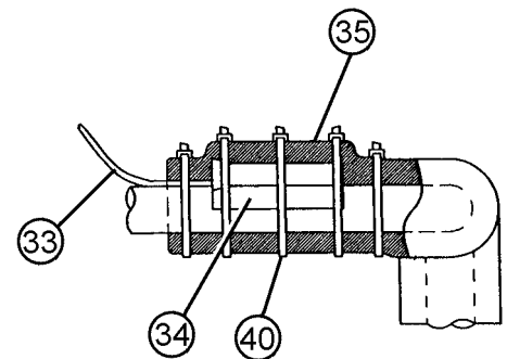
DETAILED THERMISTOR ATTACHMENT
