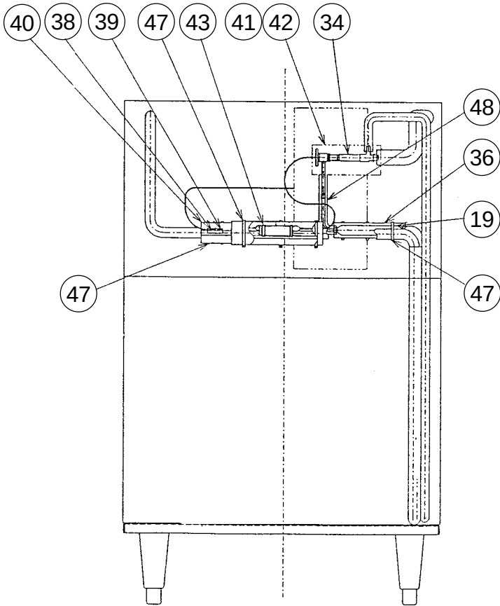
VIEW B
