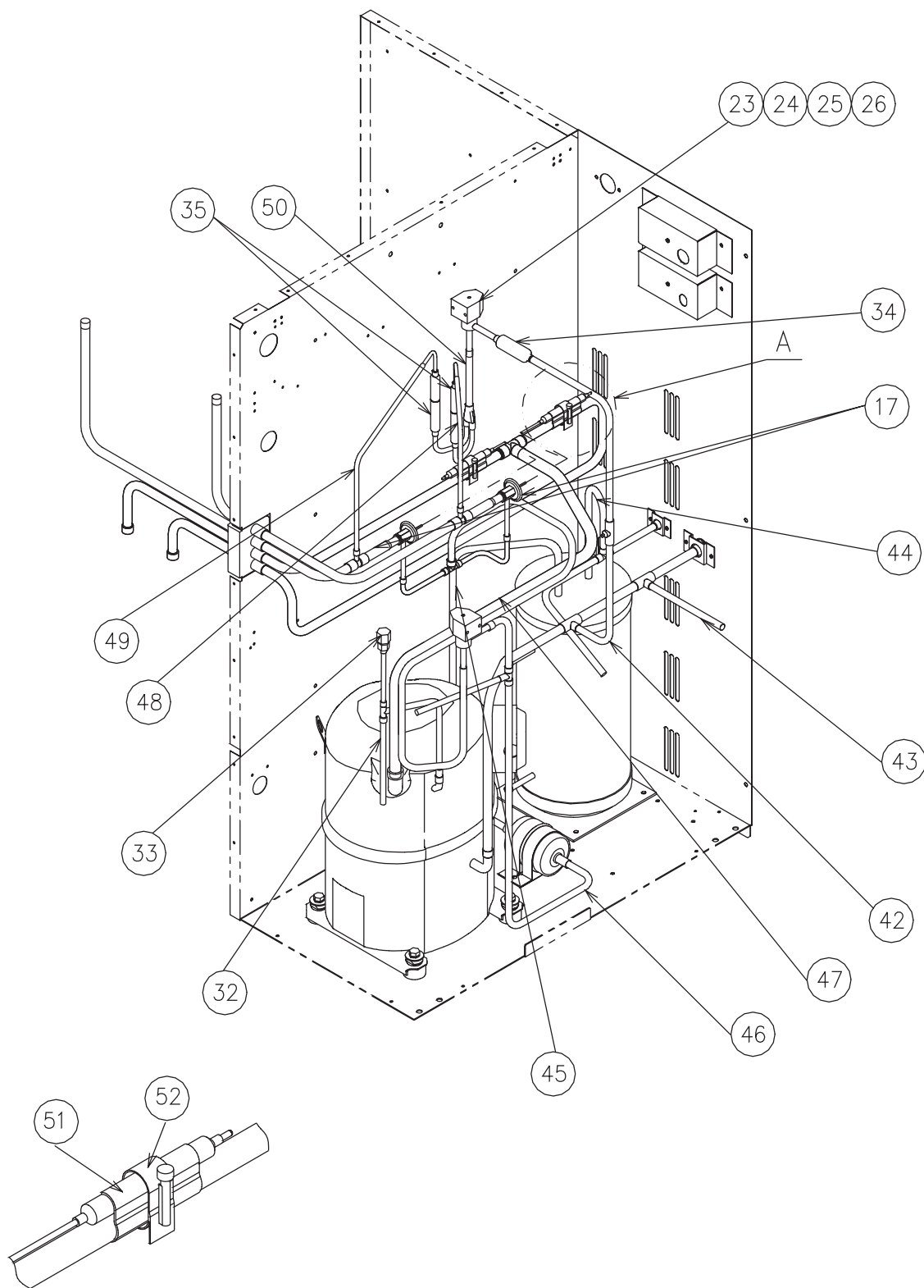
DETAIL "A" (1:2)
