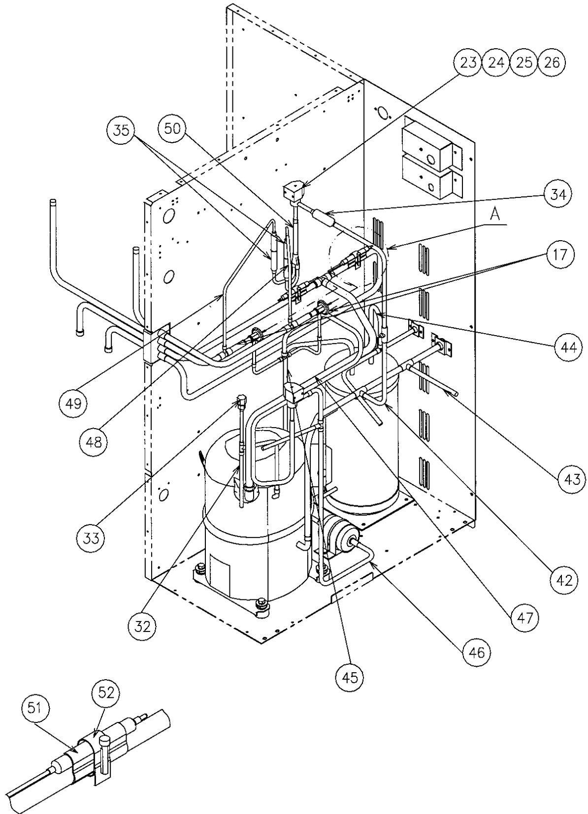
DETAIL "A" (1:2)
