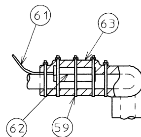
DETAILED THERMISTOR ATTACHMENT
