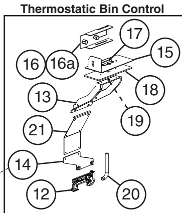
Thermostatic Bin Control
