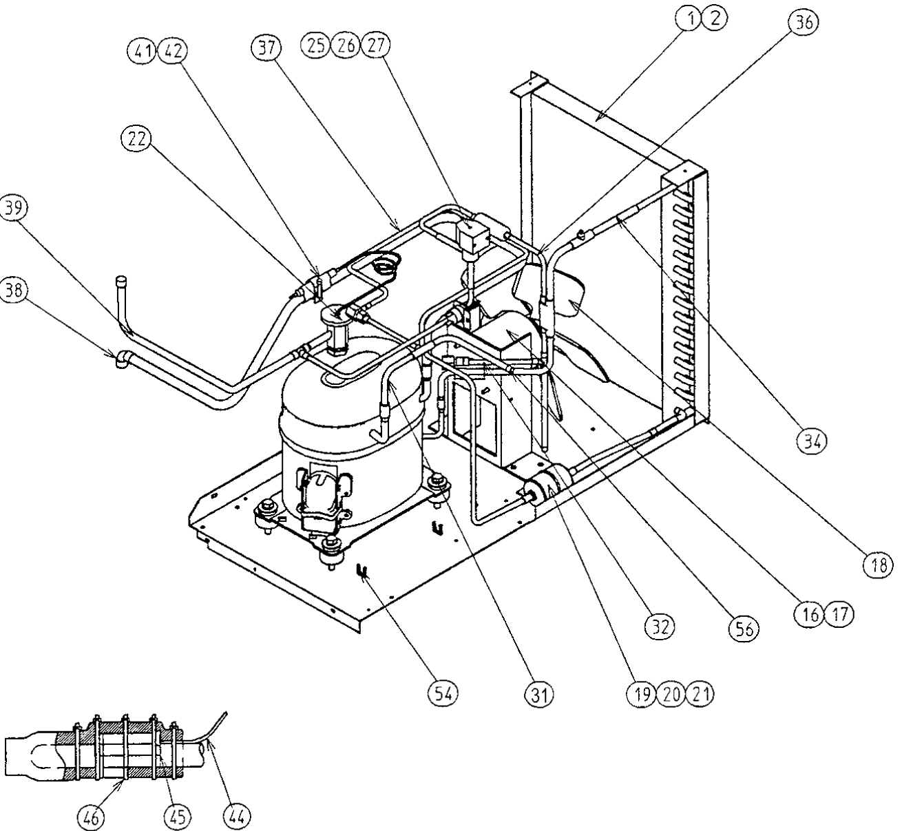
THERMISTOR ATTACHMENT
