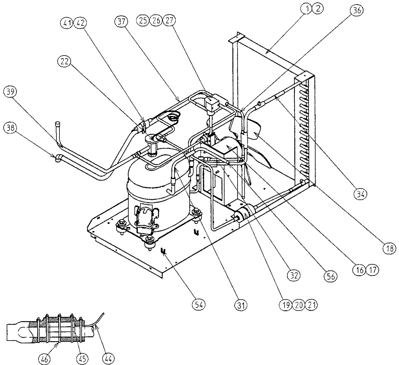
THERMISTOR ATTACHMENT
