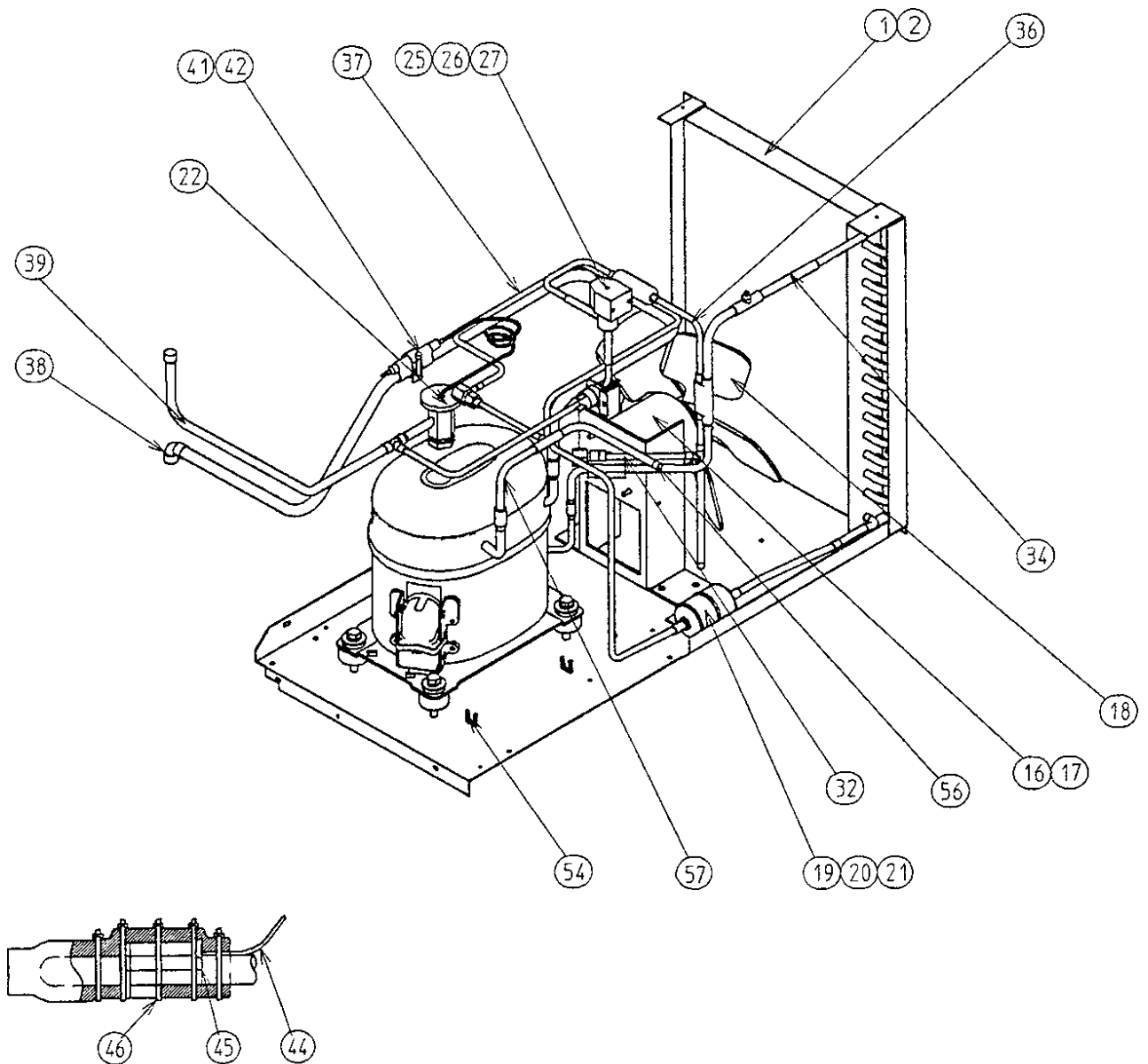
THERMISTOR ATTACHMENT
