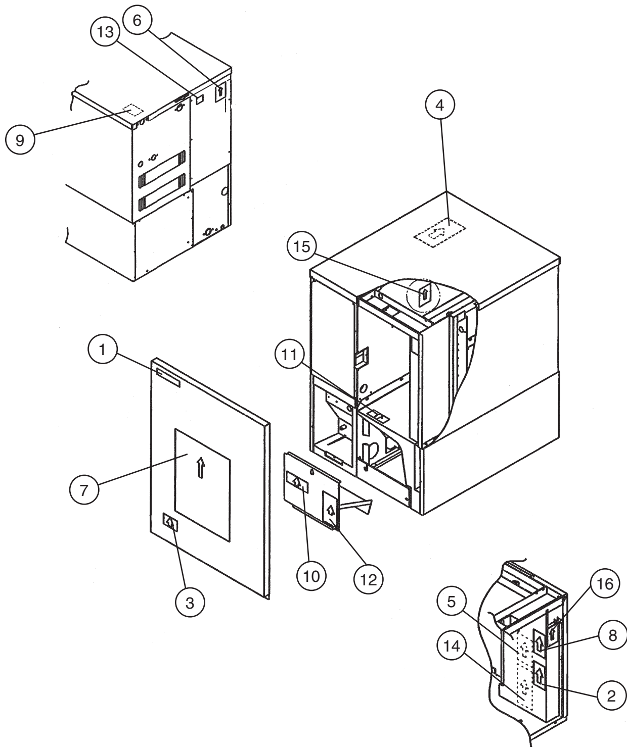
Control Box
