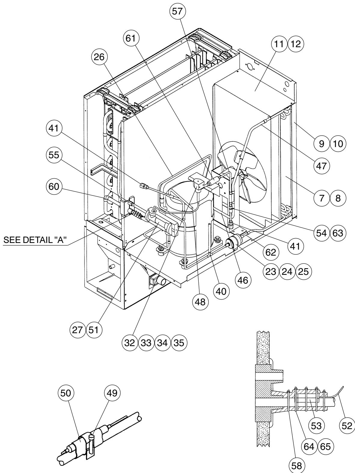
DETAILED HOLDER / EXPANSION VALVE
