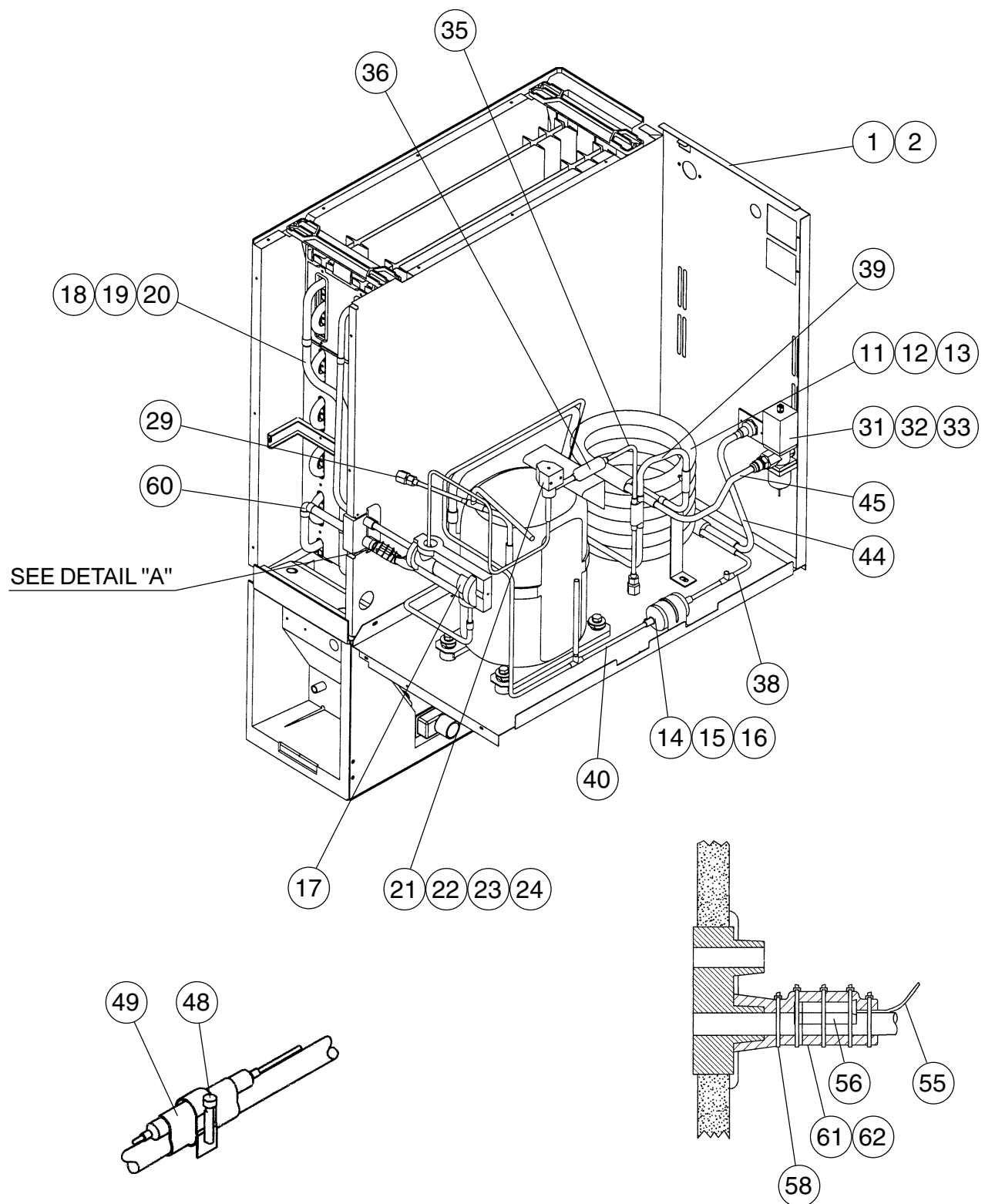
DETAILED HOLDER / EXPANSION VALVE
