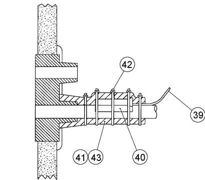
DETAIL "A" THERMISTOR ATTACHMENT
