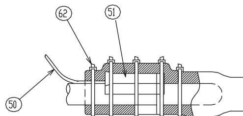
DETAILED THERMISTOR ATTACHMENT
