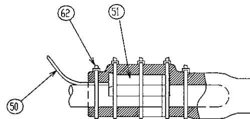
DETAILED THERMISTOR ATTACHMENT
