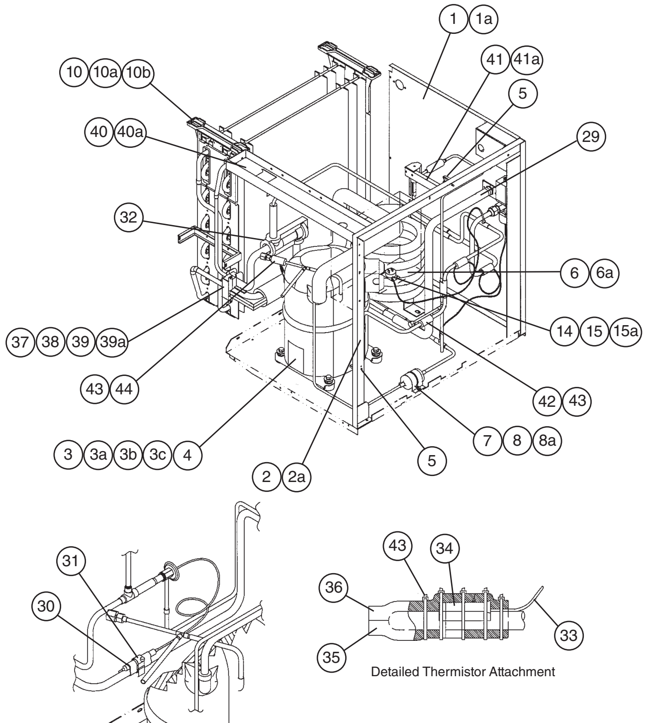
Detailed Expansion Valve Bulb Attachment
