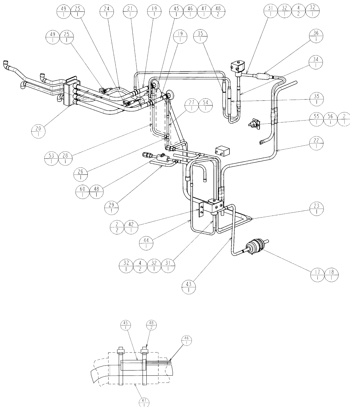
DETAILED THERMISTOR ATTACHMENT
