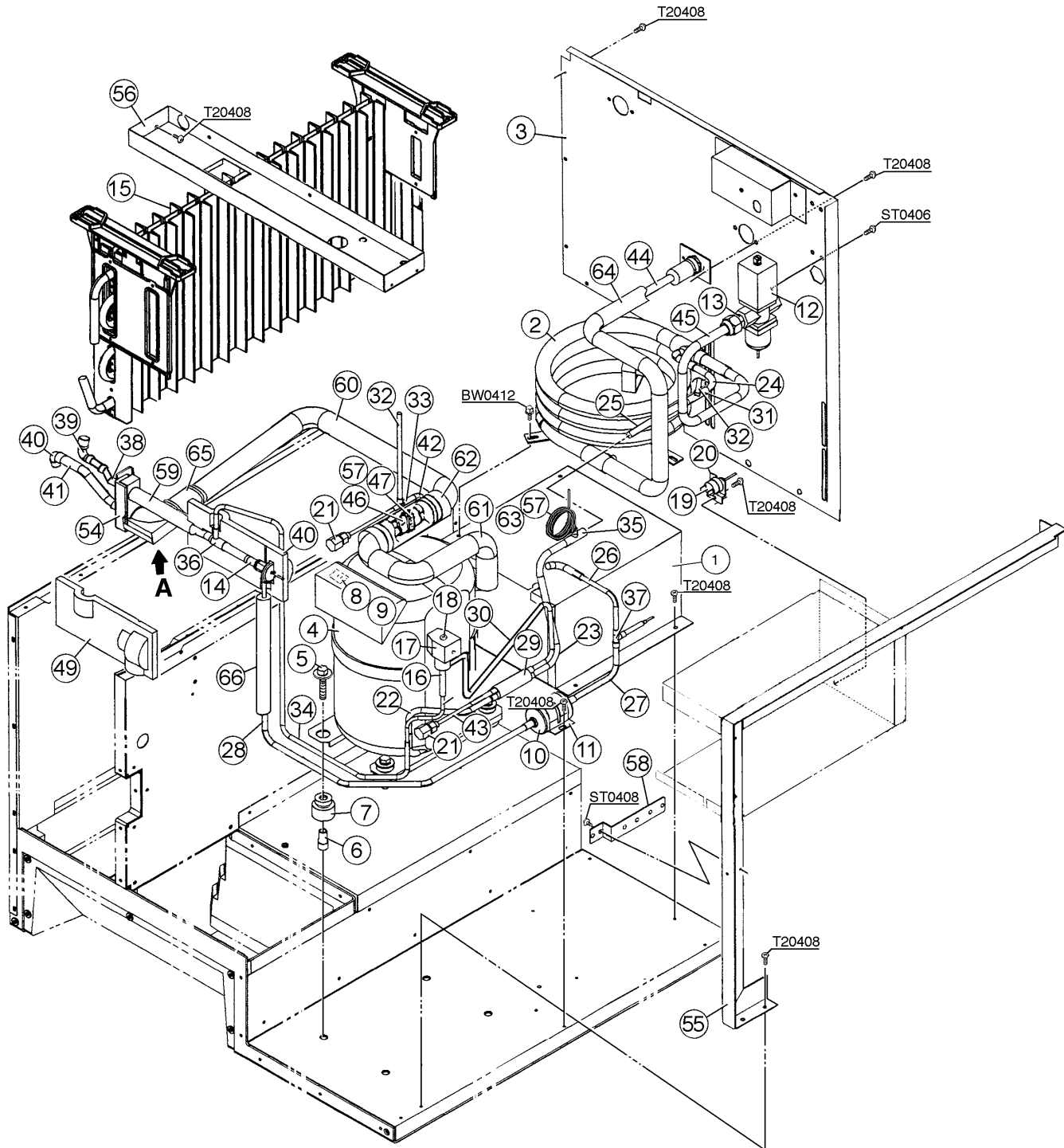
View A
