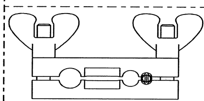
FIG. B - RE-ROUNDING TUBING
